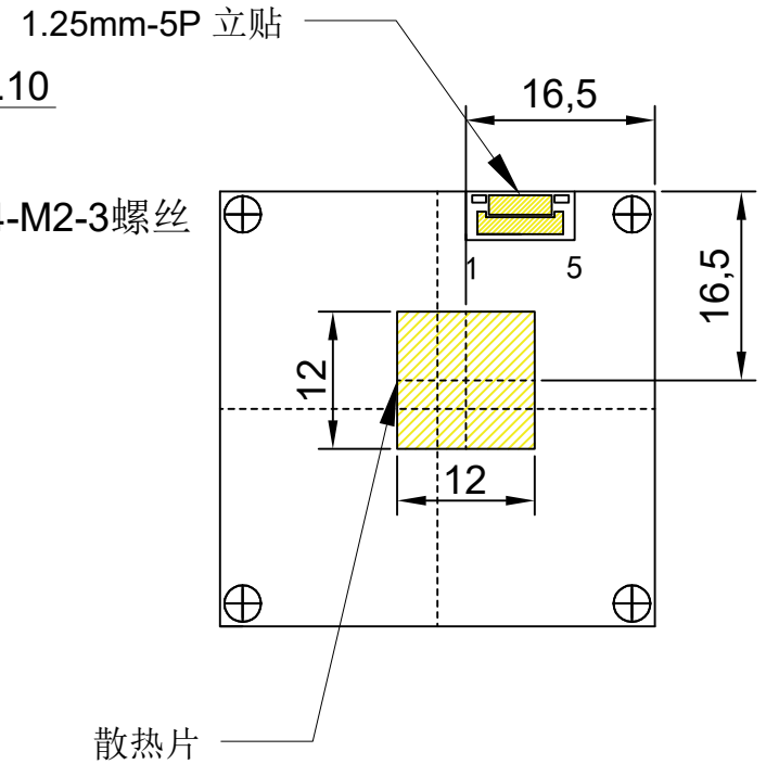
BOTTEM VIEW
